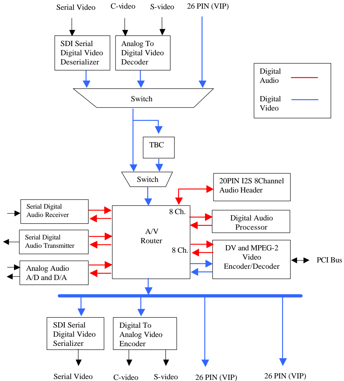
Merlin 2001 Block Diagram
